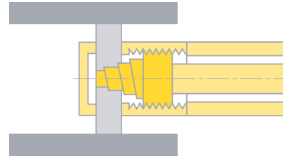
The measuring bolts with 3-line contact allows the micro-meter to align itself parallel to the contact surfaces.
